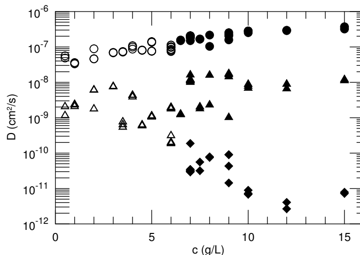
Figure 5: Effective diffusion coefficients D = \langle \Gamma \rangle / q^2 fast (circles), intermediate (triangles), and slow (diamonds) spectral modes of HPC:water. Open and closed points indicate parameters from two- and three-mode fits, respectively.
