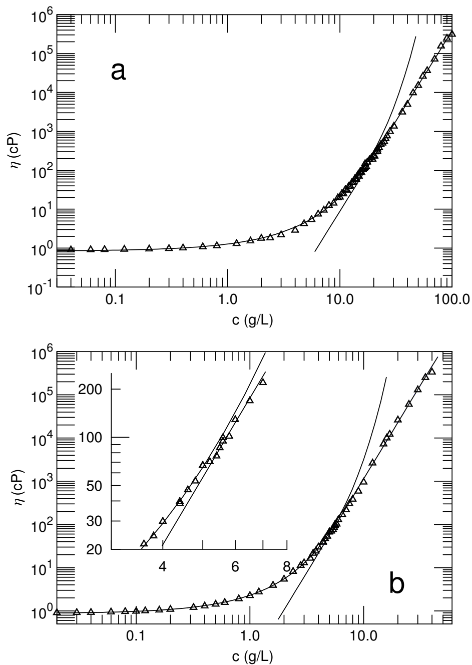
Figure 1: Viscosity against concentration of (a) 300 kDa, (b) 1 MDa, and (next page, top) (c) 1.15 MDa hydroxypropylcellulose:water, after Phillies and Quinlan[25].
