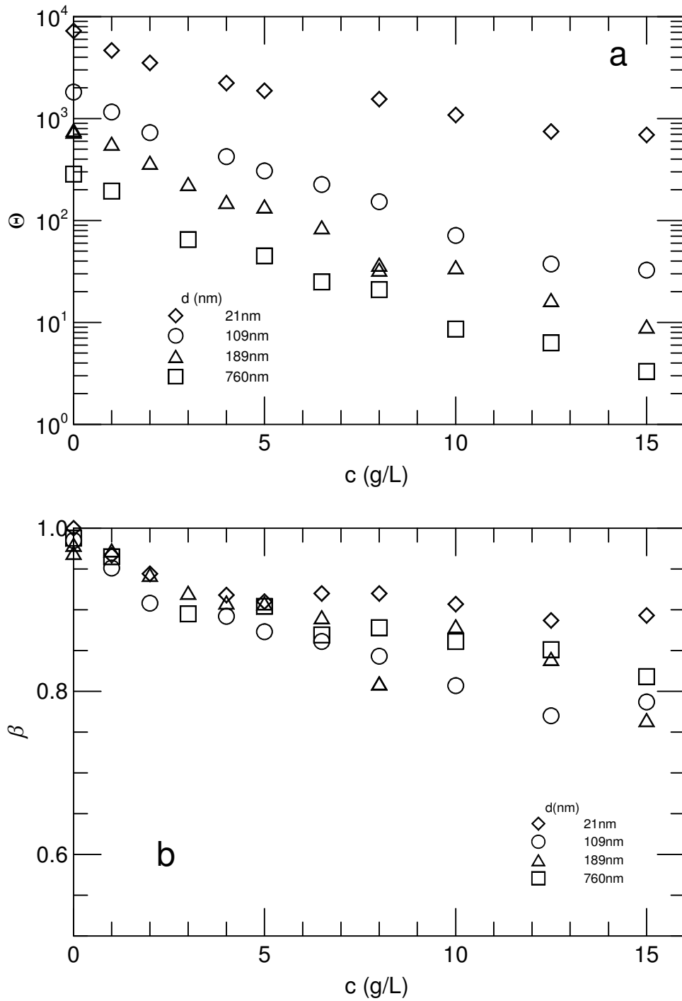
Figure 14: (a) \theta and (b) \beta as functions of polymer concentration for probe spectra of spheres in 415 kDa HPC:water.
