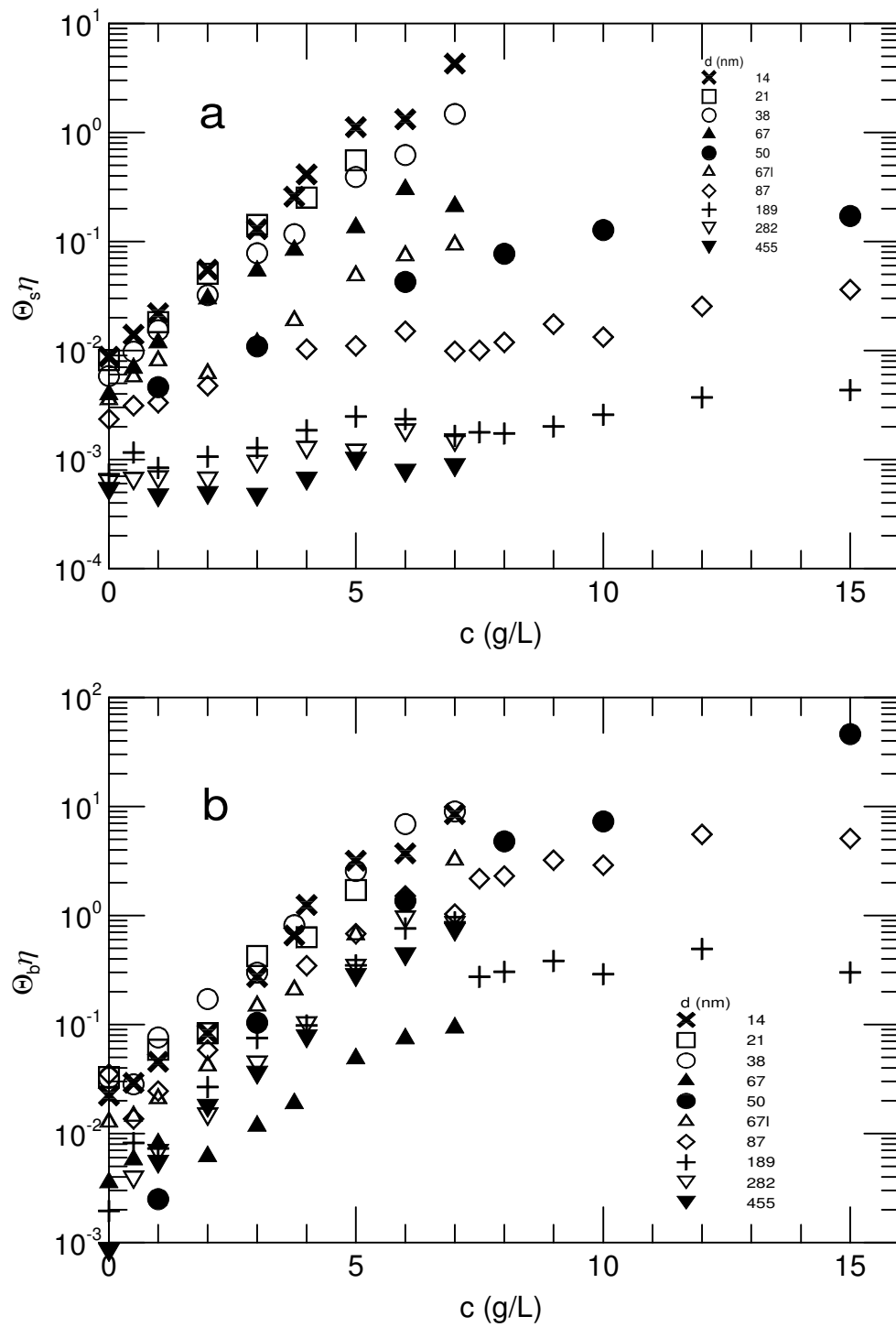
Figure 10: Correlation between decay pseudorates and the solution viscosity, from a) \Theta_s \eta and b) \Theta_b \eta against concentration for all probes studied.
