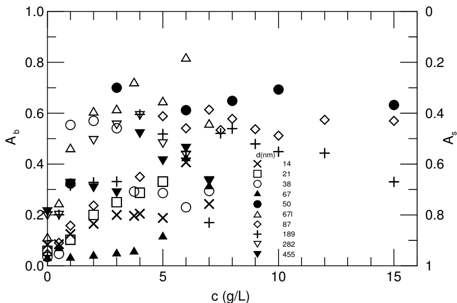
Figure 9: Relative amplitudes ( A_b + A_s = 1 constrained) of the broad (left scale) and sharp (right scale) modes for 14-455nm probes (Figure legend) as functions of polymer concentration c .
