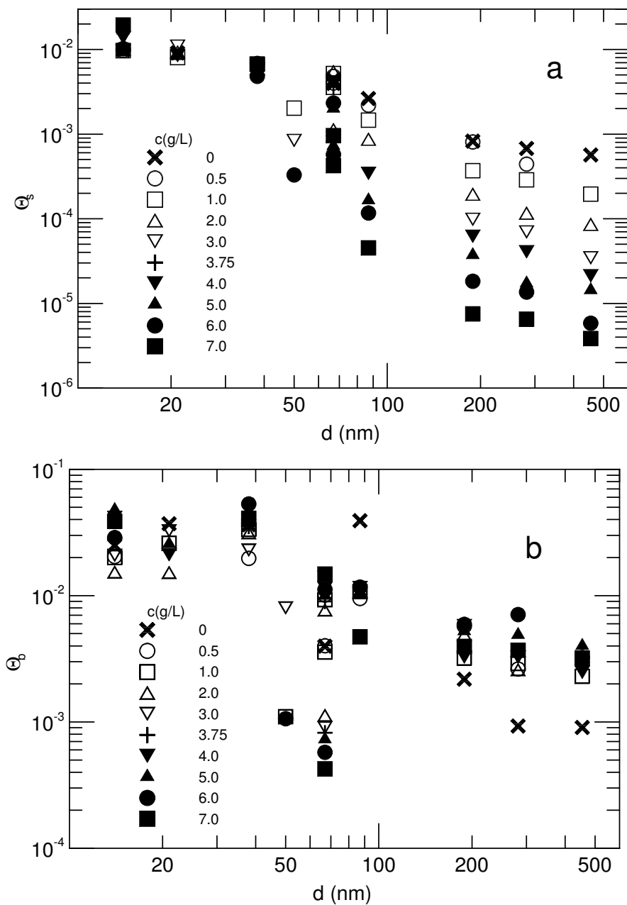
Figure 7: Relaxation pseudorates a) \theta_s and b) \theta_b of the sharp and broad modes, respectively, plotted as functions of probe diameter at each of a series of polymer concentrations c \leq c^+ , showing showing the marked difference in concentration dependences between small ( d < 50 nm) and large ( d > 50 nm) sphere behavior.
