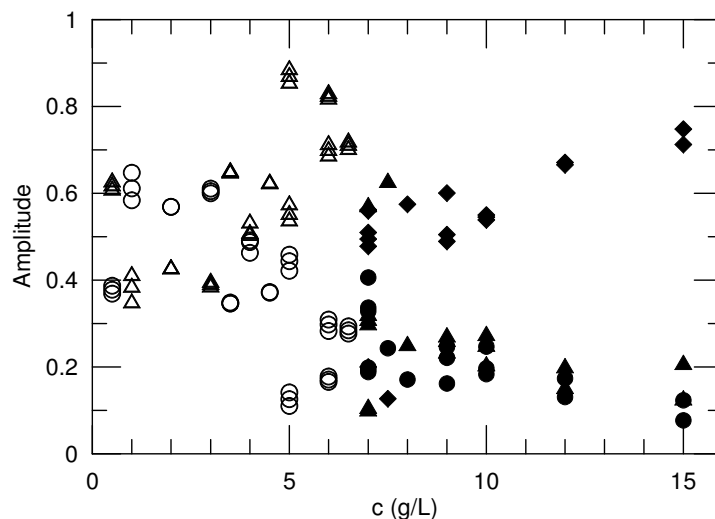
Figure 4: Relative amplitudes of the fast (circles), intermediate (triangles), and slow (diamonds) spectral modes of HPC:water as functions of HPC concentration. Open points indicate parameters from two-mode fits; filled points indicate parameters for three-mode fits.
