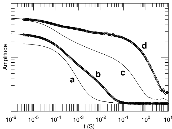
Figure 3: Renormalized spectra S(q,t) of aqueous solutions of 1MDa HPC at concentrations of (a) 1, (b) 4.5, (c) 7, and (d) 12 g/L HPC. At 4.5 and 12 g/L, points are data and line are fits to two or three stretched exponentials, respectively. For readability, these spectra were renormalized and displaced vertically relative to each other.
