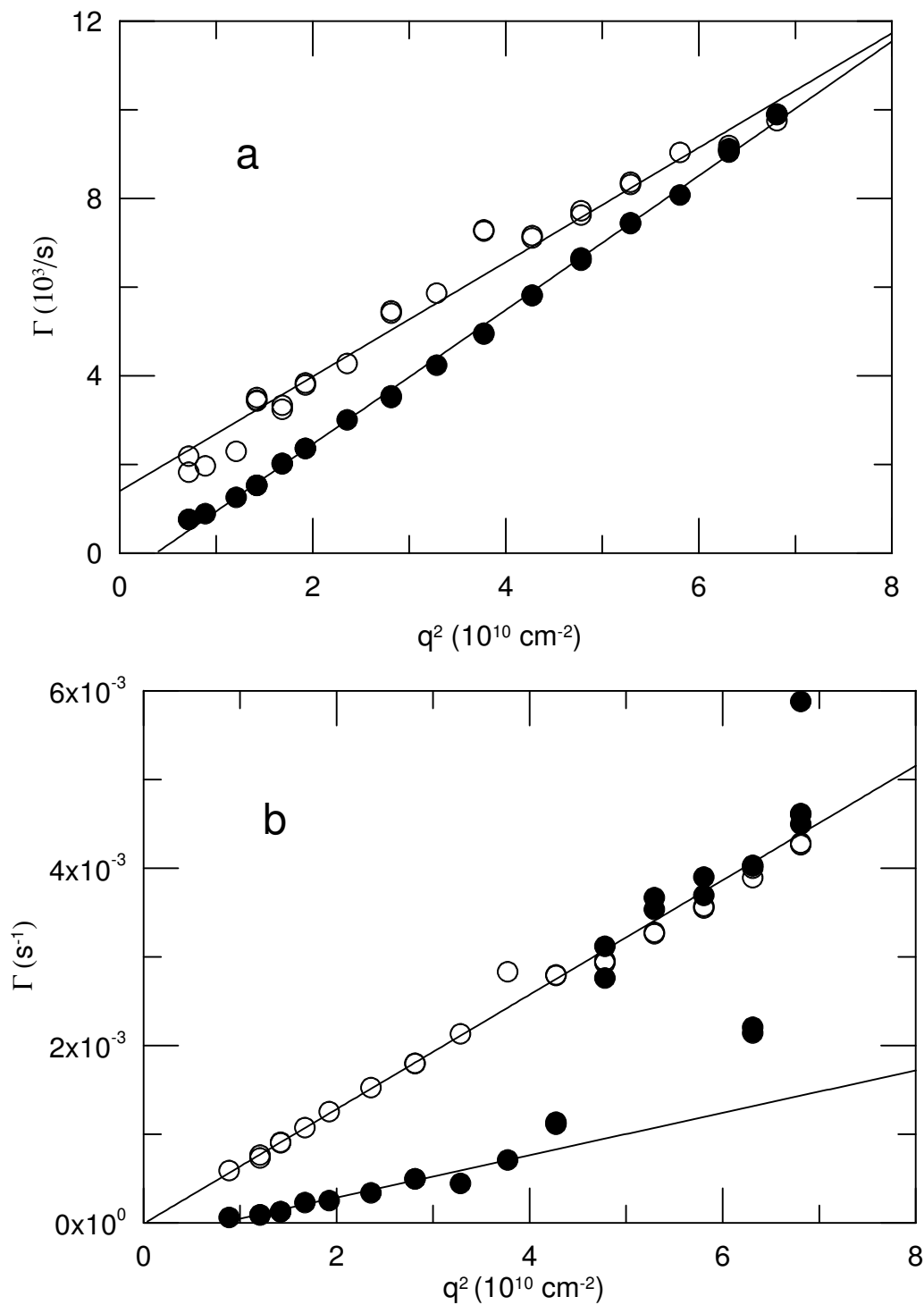
Figure 13: Mean relaxation rates \Gamma = M_0^{-1} for the sharp (open circles) and broad (filled circles) modes of (a) 87 nm probes in 5 g/L HPC and b) 20 nm probes in 4 g/L HPC.
