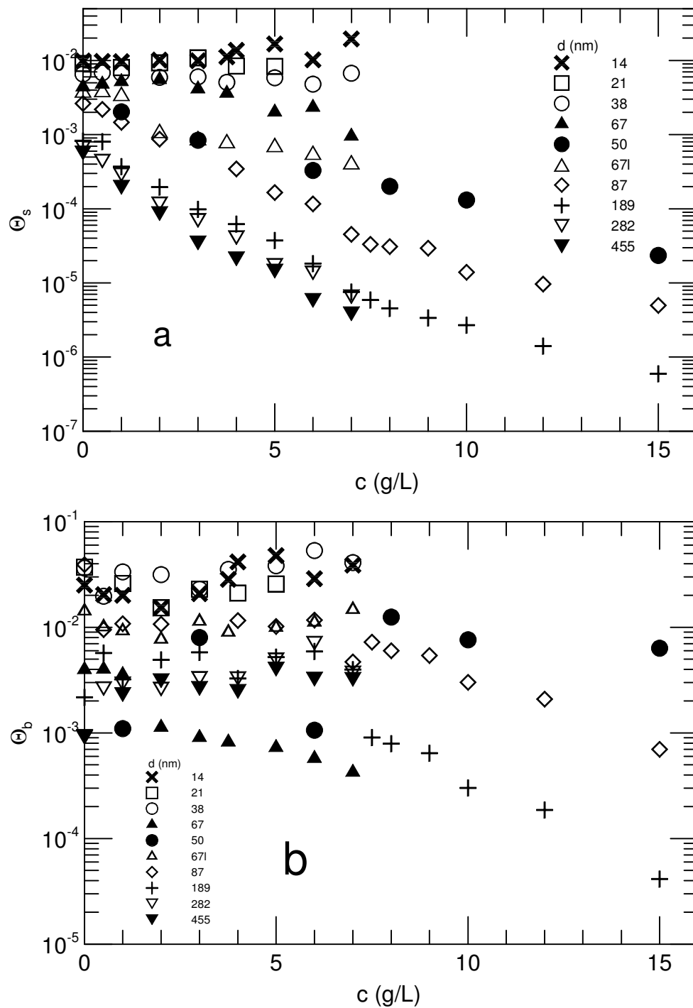
Figure 8: Relaxation pseudorates a) \theta_s and b) \theta_b plotted as functions of polymer concentration for each diameter of probe. For \theta_s , the sensitivity to polymer concentration is markedly stronger for large probes than for small probes. For all spheres, \theta_b is insensitive to polymer c until c^+ is reached. Above c^+ , \theta_b falls markedly with increasing c .
