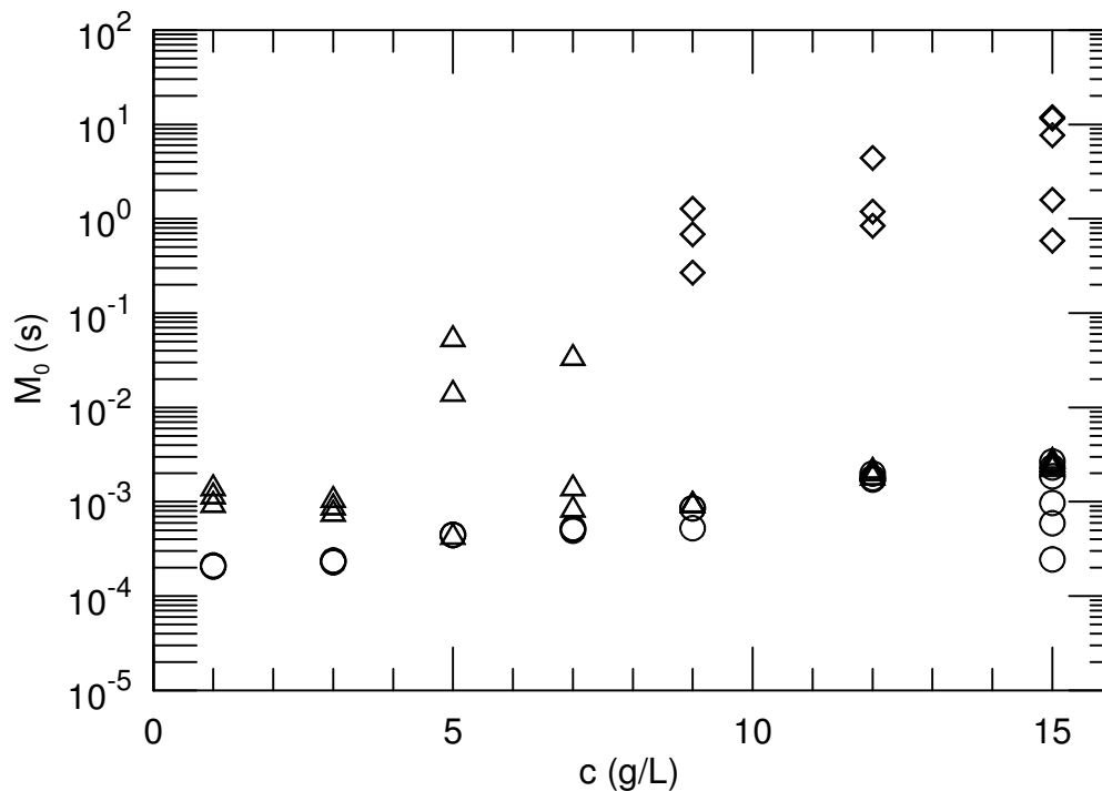
Figure 11: M_0 against c for the sharp (circles), broad (triangles), and ultraslow (diamonds) modes of 35 nm probes in HPC:water.
