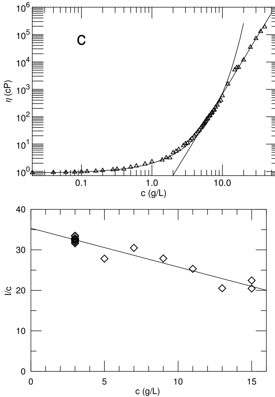
Figure 2: Normalized static scattering intensity I/c of aqueous 1MDa HPC, as a function of HPC concentration, and simple linear fit to I/c as a function of c , showing that the scattering per molecule of HPC in solution declines slowly but uniformly with increasing concentration, after O'Connell, et al.[59].
