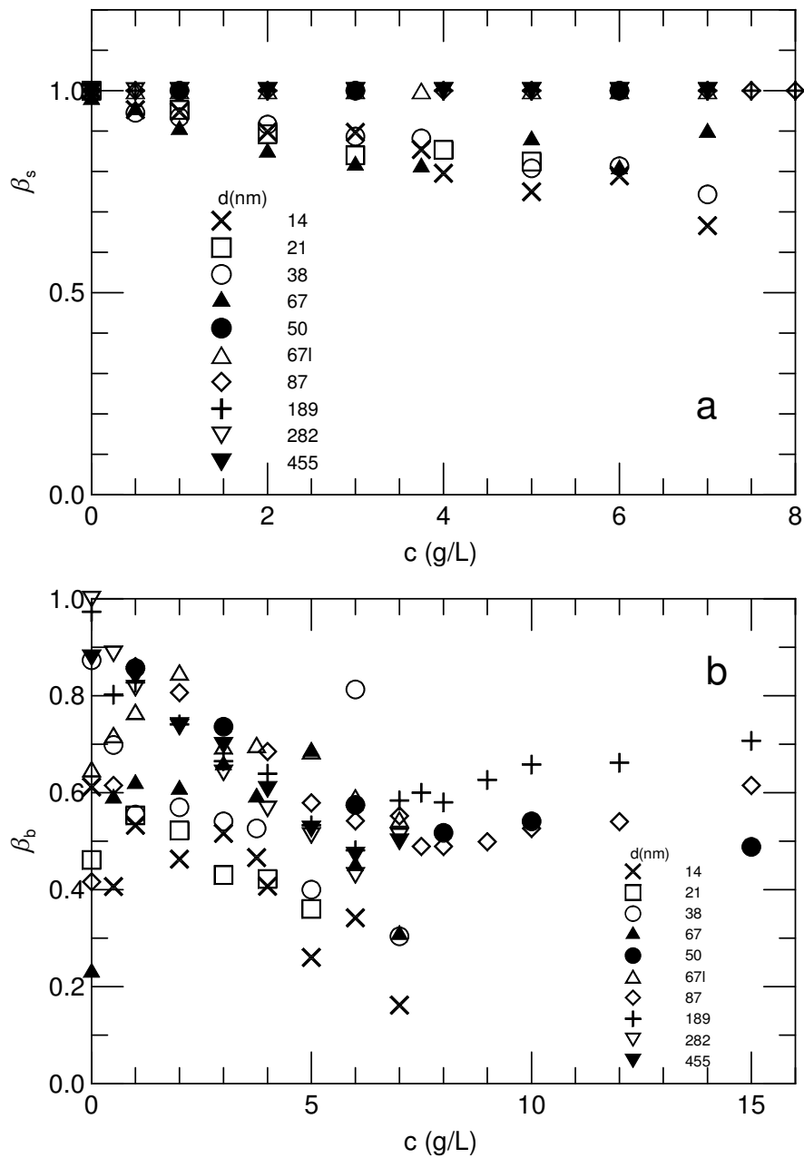
Figure 6: Spectral parameters from optical probe spectra. Stretching exponents a) \beta_s and b) \beta_b of the sharp and broad modes, obtained by fitting the spectra of small ( d \leq 67 nm) probes to a sum of two stretched exponentials and fitting the spectra of large ( d \geq 67 nm) spheres to the sum of a stretched exponential and a pure exponential (for which \beta_s = 1 applies). Fits to 67nm sphere spectra are reported treating it both as a small "67" and as a large "671" probe. For c > 8 g/L, only large spheres for which \beta_s \equiv 1 (not plotted) were studied.
