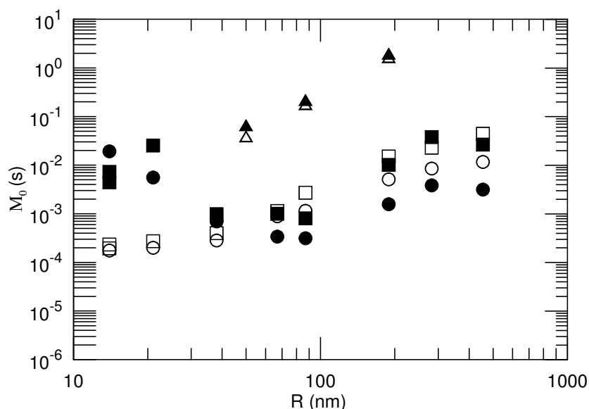
Figure 12: Dependence of the sharp (open points) and broad (filled points) modes of polystyrene latex probes on probe diameter R at concentrations 2 (circles), 4 (squares), and 15 (triangles) g/L HPC.
