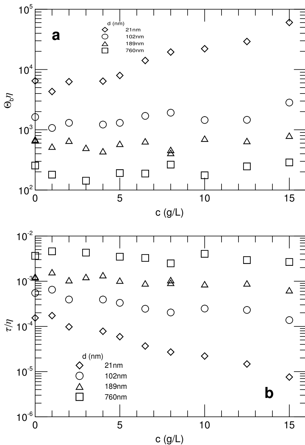
Figure 15: Relation between decay pseudorate and pseudotime and solution viscosity, for probes in HPC: water[27], namely a) \theta_s \eta and b) \tau/\eta against c .
